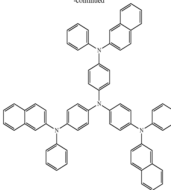
2-TNATA
